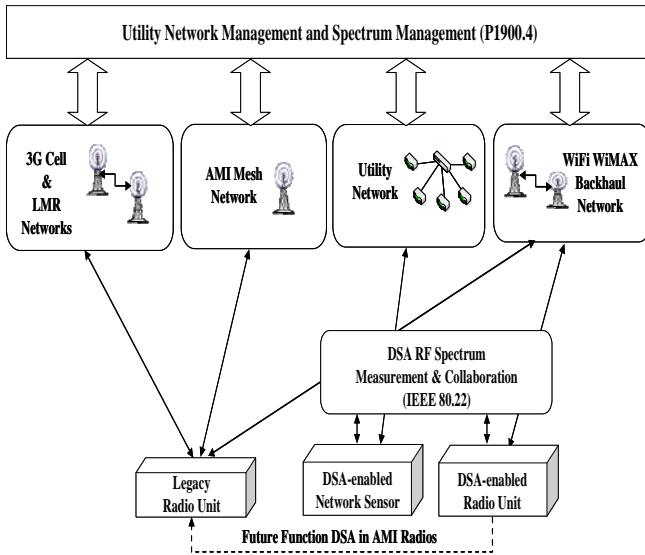
Figure 1.0 Spectrum management and DSA in a Utility Network
